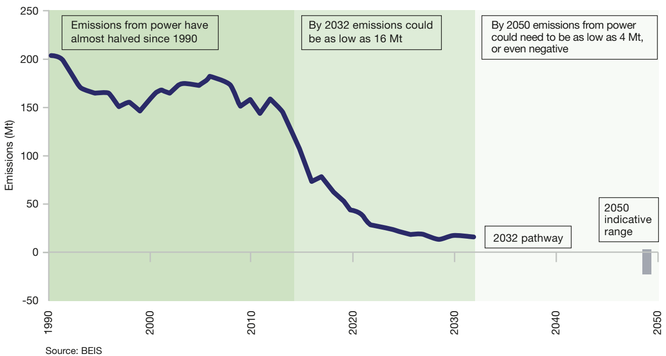
Figure 25: Actual and projected power sector emissions, taking into account the clean growth pathway, 1990-2050
